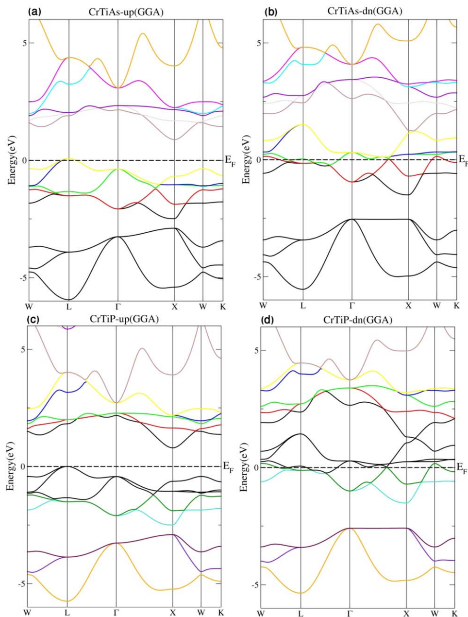
Figure 4. The band structure of CrTiZ ( Z = \text{As, P} ) compounds in GGA and mBJ approximations for two up and down spins.
