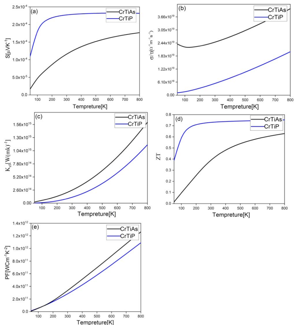
Figure 6. Temperature dependence of the (a) Seebeck coefficient, (b) electrical conductivity, (c) Thermal conductivity (d) figure of merit (ZT), and (e) power factor (PF) in the range of 50–800 K for CrTiZ (Z = As, P) compounds.
