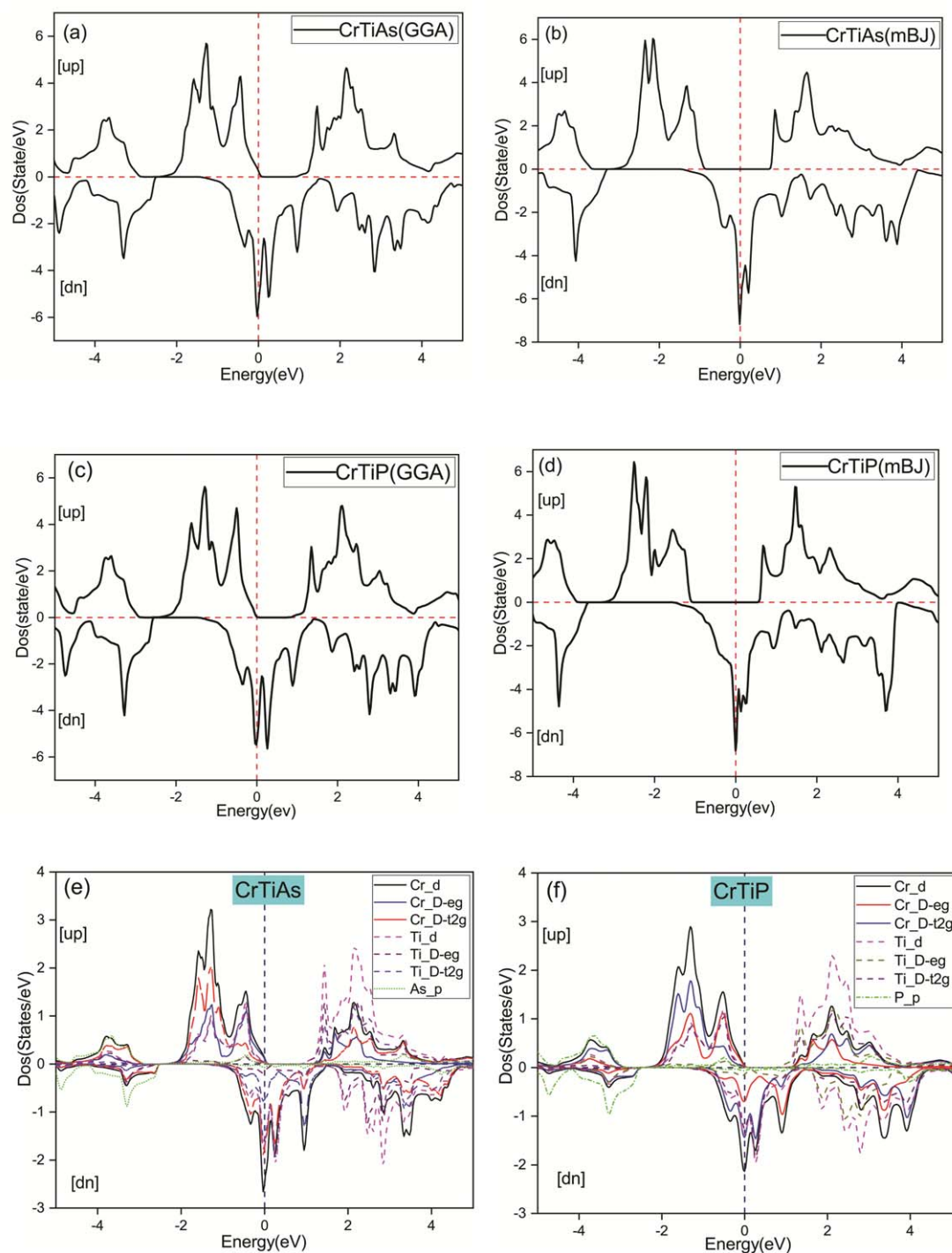
Figure 3. (a)–(d) The DOS of the CrTiZ (Z = As, P) compounds by GGA and mBJ approximations, and (e), (f) are the partial DOS for two up and down spins.
